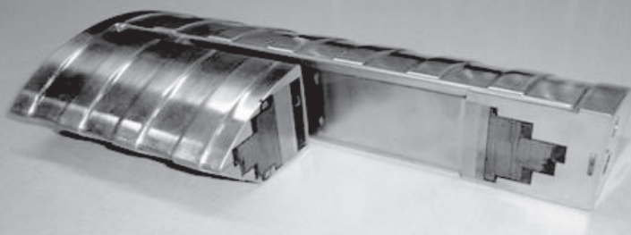
MgB2 rotor coil for 2 MW high speed, 15000 rpm motor
